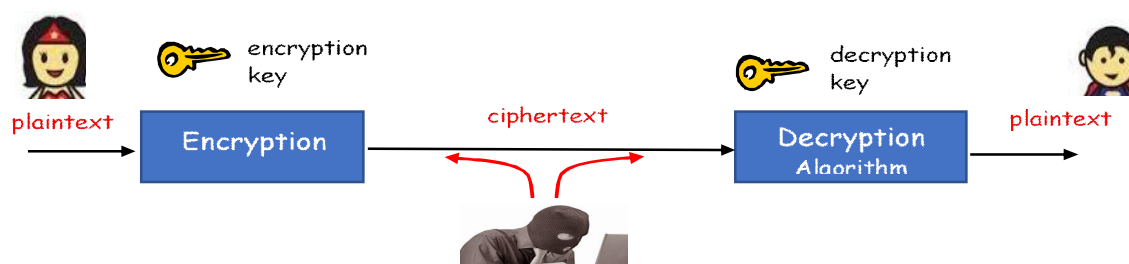
Fig.2.Cryptographic illustration
